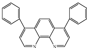
BPhen
